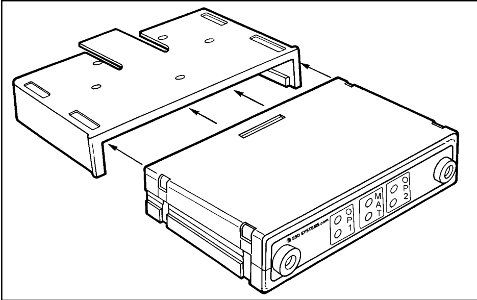
Figure 1. ESD Systems.com 41137 Dual Operator Workstation Continuous Monitor.
