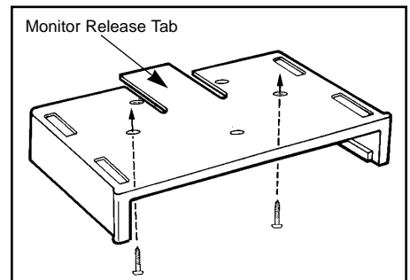
Figure 2. Installation of mounting bracket.
